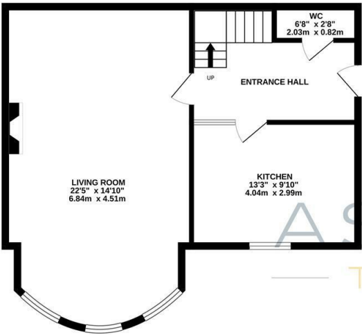
GROUND FLOOR 601 sq.ft. (55.9 sq.m.) approx.
